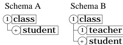
Fig. 4. Incompatible schemas
