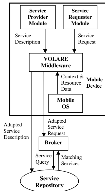
Figure 1: The VOLARE architecture
