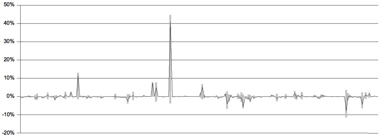
Figure 4. ArgouML: Deletions
