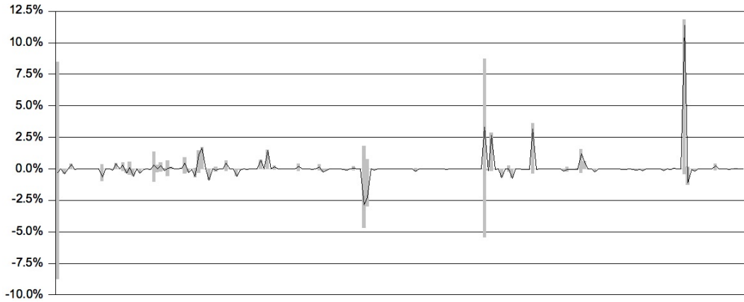
Figure 9. SquirrelL: Deletions
