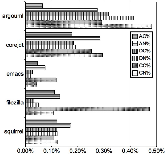
Figure 12. Smoothed Summary of the Results
