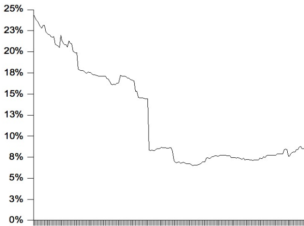
Figure 2. ArgoUML's size during 200 weeks
