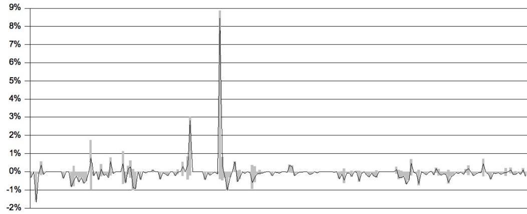
Figure 10. SquirrelL: Additions
