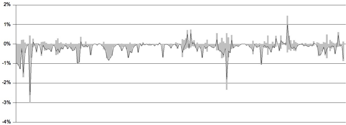
Figure 5. ArgouML: Additions
