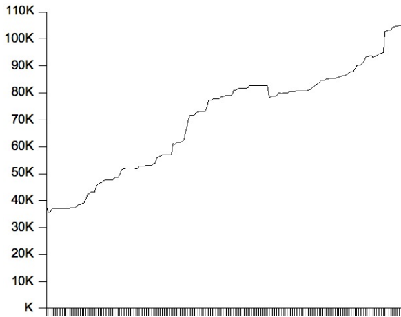
Figure 7. Squirrel's size during 200 weeks
