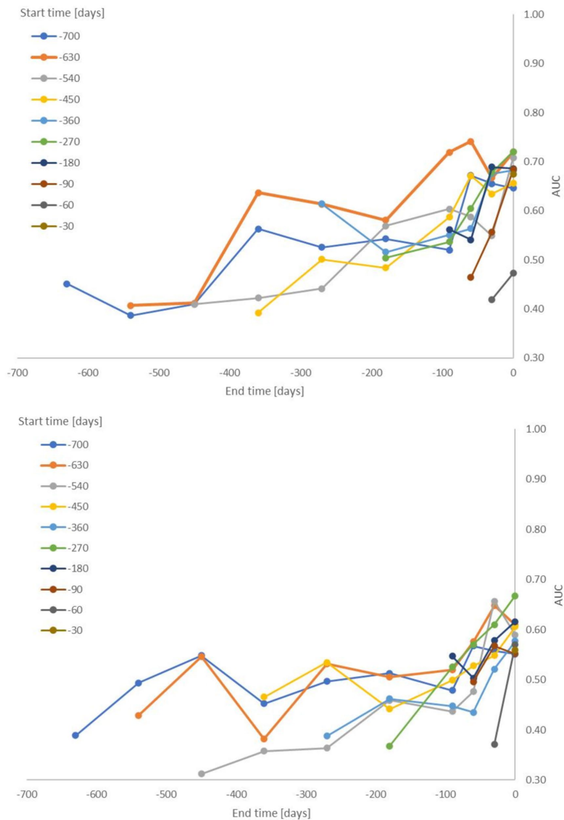
Fig. 3 Model performance as a function of start and end times. The top figure shows the AUC for the terms model and the bottom figure for the categories model. The start and end times correspond to the duration of time in advance of GP referral date. Different lines correspond to different start ( T_1 ) times and the dots on each line correspond to different end ( T_2 ) times. Each dot represents the average of 10 runs. Standard deviation is equal, on average, to 0.01 (1.8% of the average AUC)
