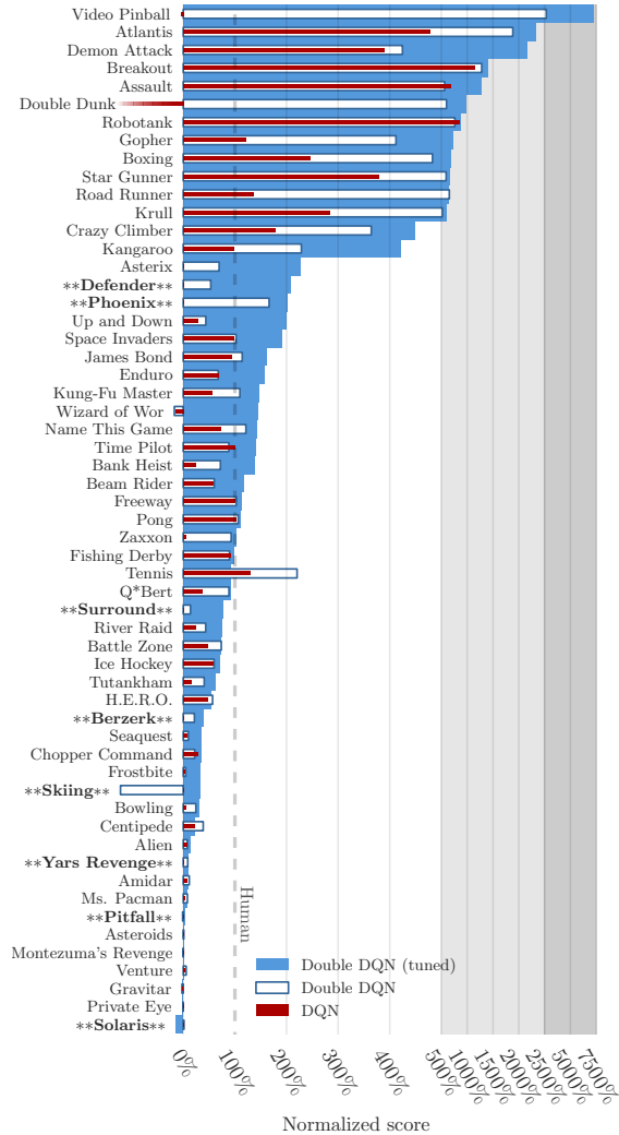
Figure 3: Normalized scores on 57 Atari games, tested for 100 episodes per game with human starts. Compared to Mnih et al. (2015), eight games additional games were tested. These are indicated with stars and a bold font.
