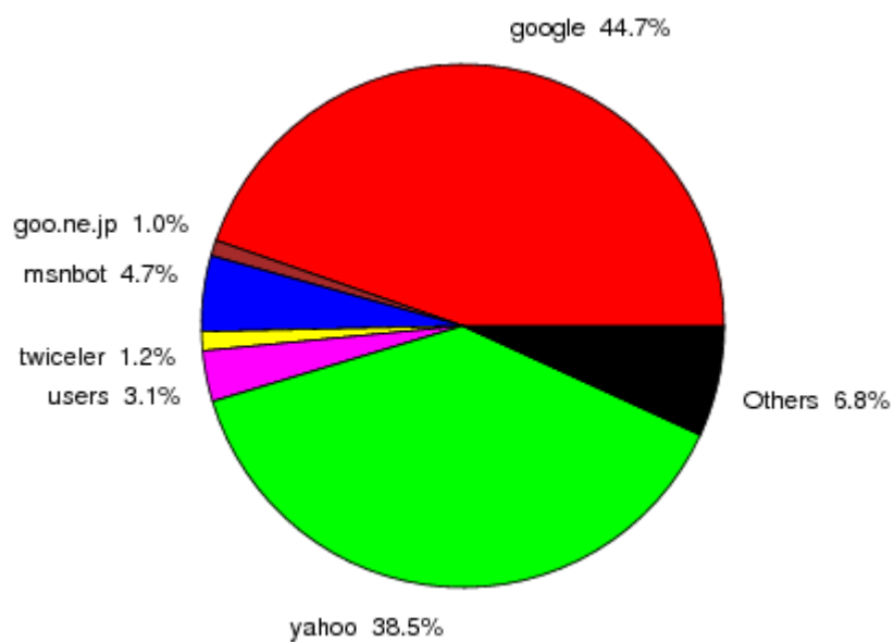
Figure 5. Web robots used to download GP papers (17 Nov 2008 to 17 Nov 2009) Human activity, “users” 11 187, is a small fraction of the total 356 644.
