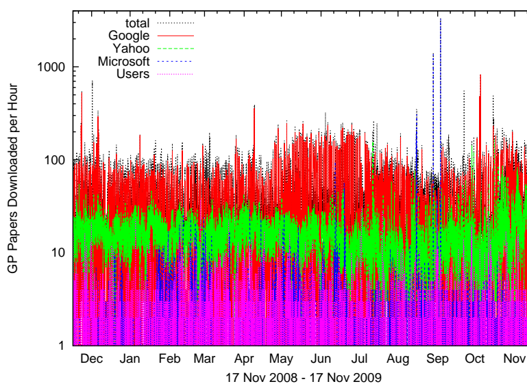
Figure 6. A year’s use of the GP bibliography links to papers (black) and broken down by major web bots and users (colour). The infrequent peaks of very high activity (max 3296) are less emphasised by the log vertical scale.
