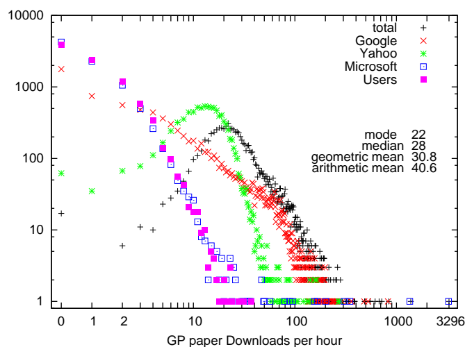
Figure 7. GP paper down loads per hour (17 Nov 2008 to 17 Nov 2009). Note log scales. User activity ■ msnbot □ and Google bot × follow approximate power laws ( x^{-3} and x^{-1} ) The total + is more parabolic suggesting a log-normal distribution. Yahoo * has a similar shape, hinting it is also the combination of a few underlying power laws. All distributions are much wider than would be expected if downloads were random independent events. Notice there are only 17 hours in the year with no activity (perhaps due to server outage).
