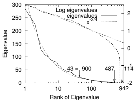
Fig. 4. 942 Eigen values of the GP-bib connectivity matrix C .
