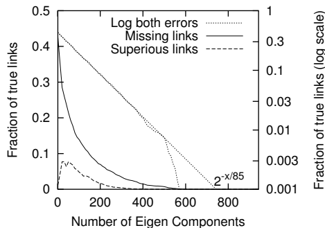
Fig. 5. Accuracy of reconstructed giant component of GP coauthor graph.
