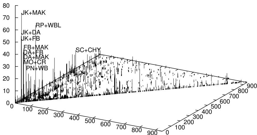
Fig. 3. Number of coauthored / coedited GP papers in the giant connected component of the GP-bib by coauthor pairings, cf. Figure 2. Prolific pairings are annotated with the coauthors' initials. To avoid clutter, only collaborations are shown, i.e. the diagonal and the lower part of C are not plotted.
