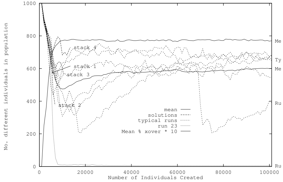
Figure 18: Number of different individuals in stack populations and proportion of subsequent duplicates produced by crossover in stack selected runs.
