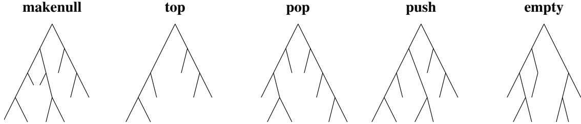
Figure 1: One Individual – One Program: Five Operations – Five Trees
