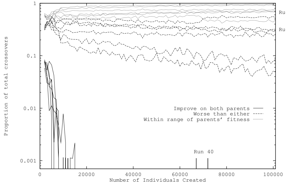
Figure 30: Proportion of crossovers that produced offspring fitter than both parents, worse than both or neither. Six typical stack runs.
