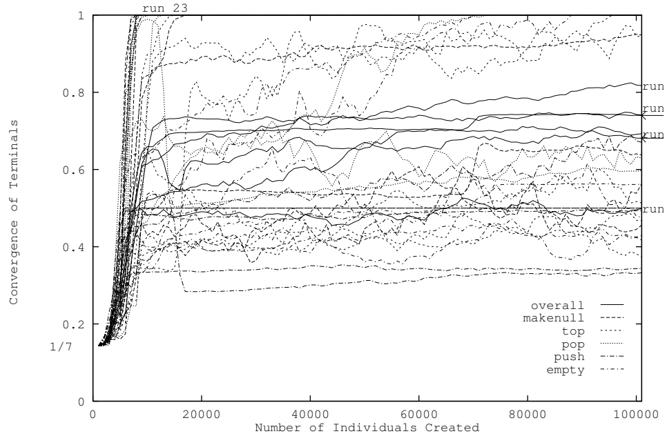
Figure 26: Evolution of (\text{Terminal Concentration})^2 in each operation tree, for six typical stack runs and run (23).
