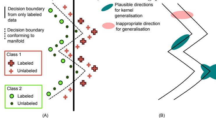
Fig. 1: Desirable properties of a learning algorithm, with respect to a manifold. (A) Knowledge of the underlying manifold structure of data can improve classification accuracy. Here unlabelled data can be used to discover the underlying shape of the manifold improving classification accuracy. (B) Given a manifold ( black ) an ideal classifier should generalise strongly in directions tangent to the manifold ( blue ) and generalise poorly with respect to directions orthogonal to the manifold ( pink, top ).
