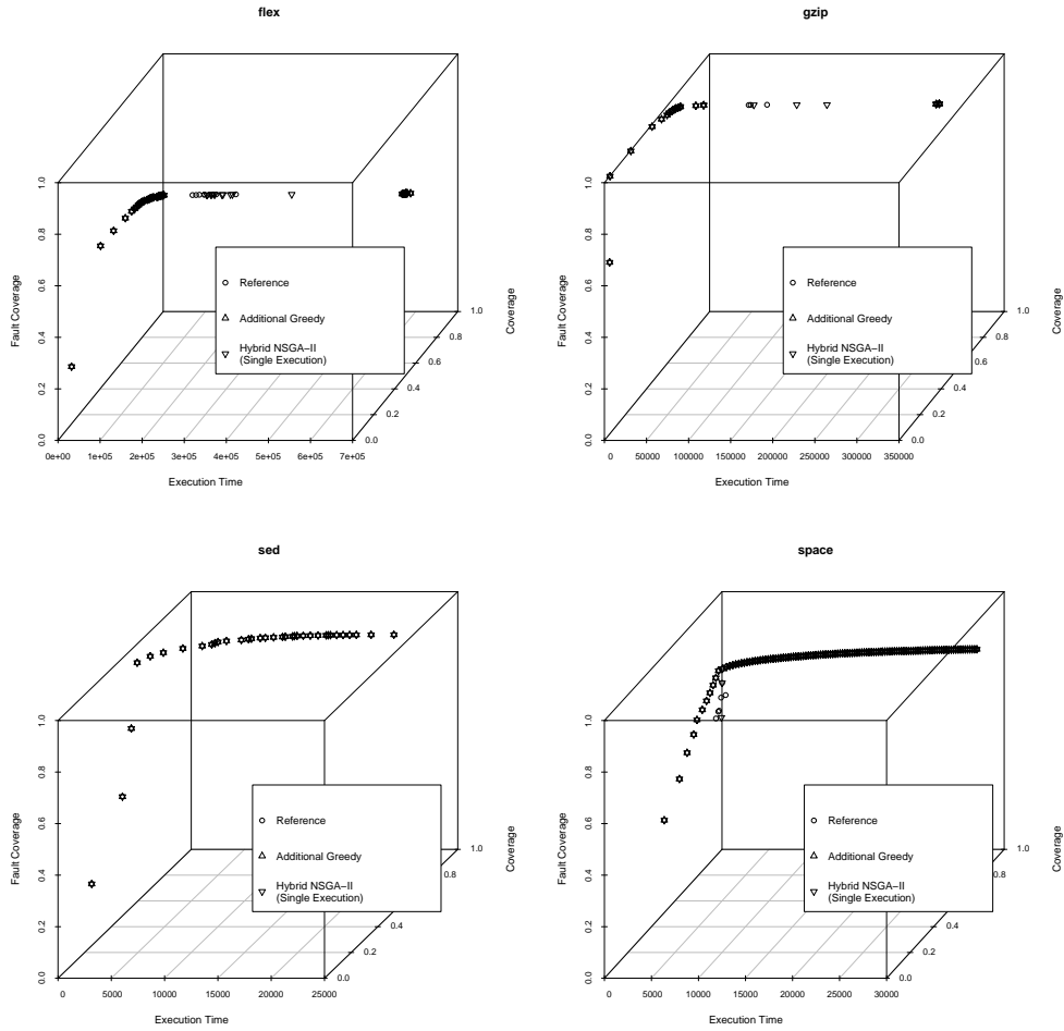
Figure 3: Plots of Pareto frontier for three objective formulation. Programs with fault-history show an elbow-point where the rates of both coverages change.
