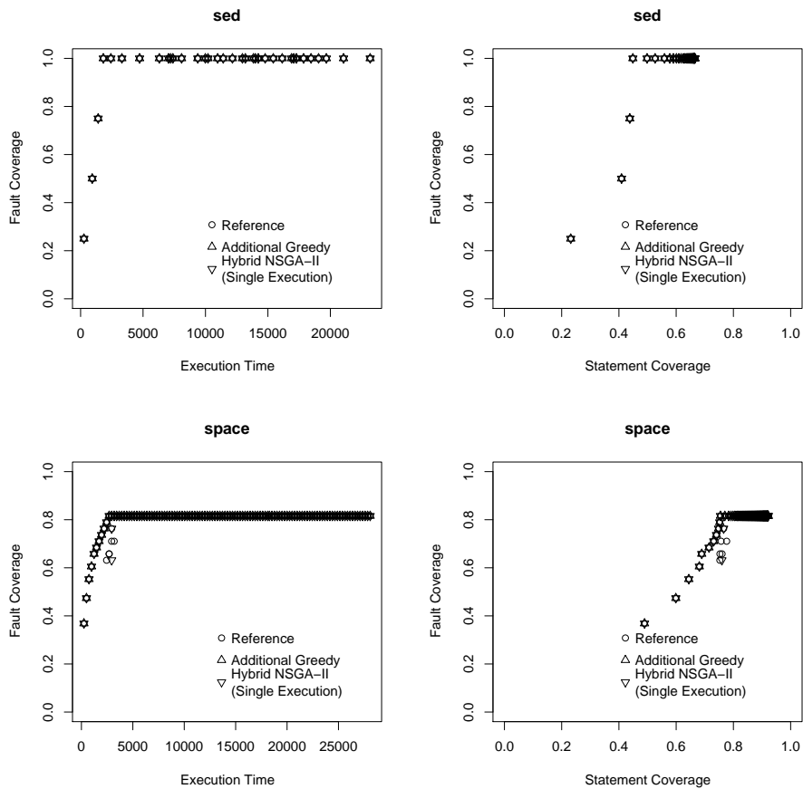
Figure 5: Two-dimensional projections of Figure 3 for sed and space . It can be observed that the fault coverage is often maximised before the statement coverage is fully maximised.
