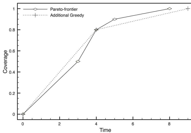
Figure 1: Comparison between the Pareto frontier and the results of the additional greedy algorithm from the test data shown in Table 1
