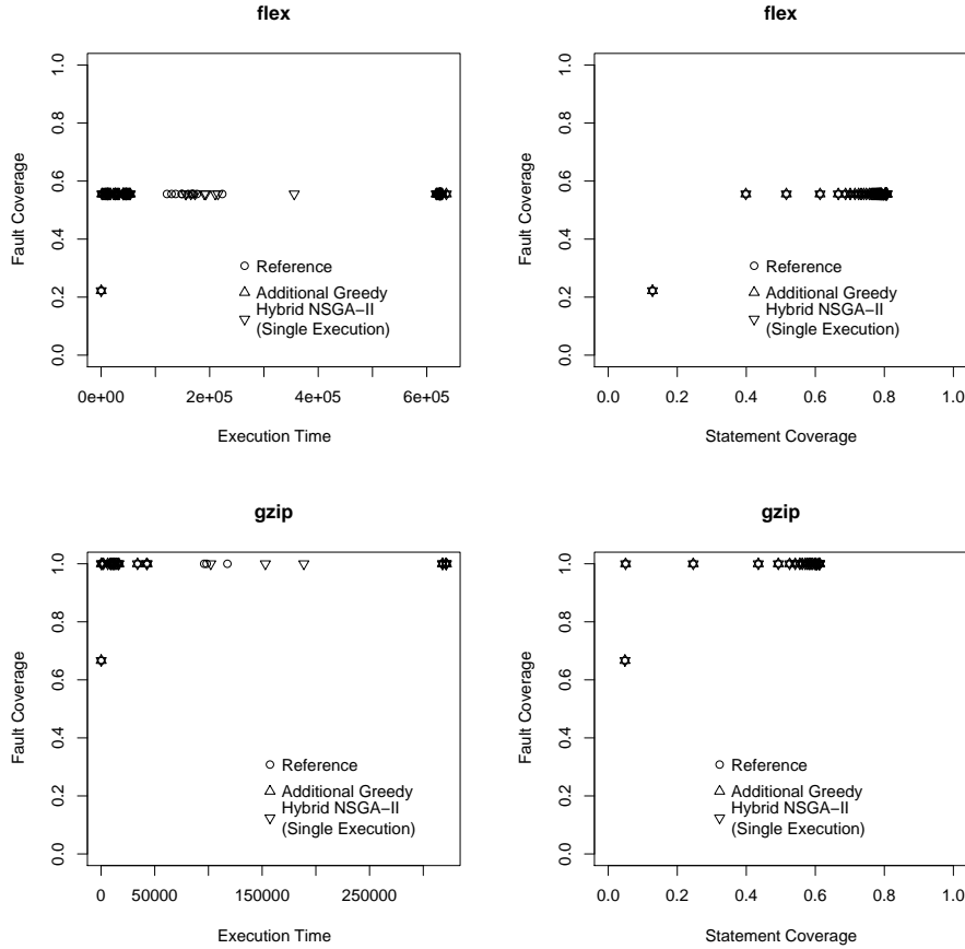
Figure 4: Two-dimensional projections of Figure 3 for flex and gzip . It can be observed that the fault coverage is often maximised before the statement coverage is fully maximised.
