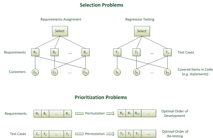
Fig. 5. Requirements Selection & Regression Testing
