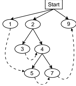
Figure 1. A small program and its dependence graph
