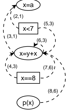
Figure 4. Dynamic data dependence graph for figure 2. Control dependence edges are omitted for readability
