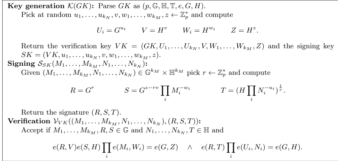
Fig. 1. Structure-preserving signature scheme for messages in \mathbb{G}^{k_M} \times \mathbb{H}^{k_N} .
