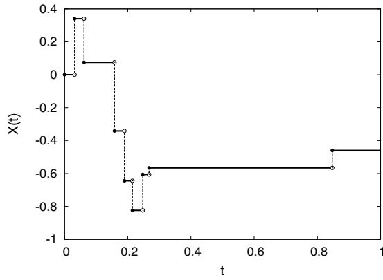
FIG. 1. Realization of a CTRW with exponentially distributed waiting times ( \gamma_t=0.1 ) and normally distributed jumps ( \mu=0 and \sigma=\sqrt{0.2} ). The probability density function p_X(x) of X(1) is plotted in Fig. 2, top left.
