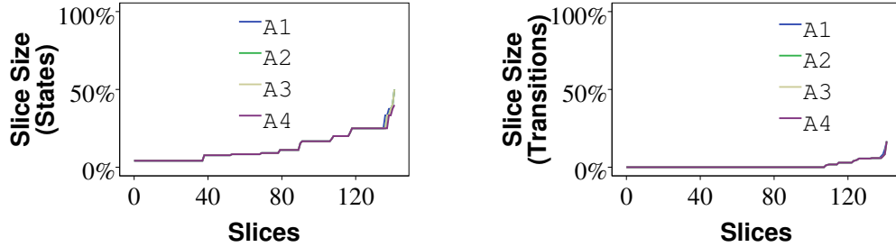
Figure 8: All slice sizes for Algorithms A_1 , A_2 , A_3 and A_4 using all possible ignore sets containing all but one ( n - 1 ) events.
