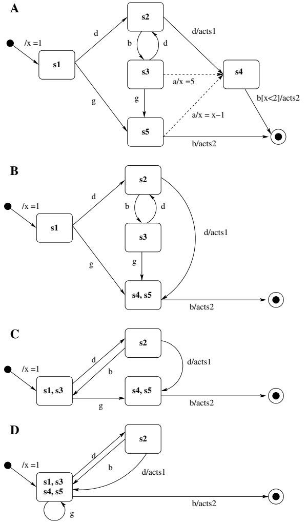
Figure 6: This example illustrates the roll of constant propagation and state merging in the current implementation of model projection. Applying basicSlice to EFSM A using ignore set \mathcal{I} = \{a\} removes the two dashed transitions from EFSM A. EFSM B shows the results of constant propagation, which replaces the guard x < 2 with “True,” and then the R-merging of states s_4 and s_5 , which is enabled by the constant propagation. EFSM C shows the result of the additional R-merging of states s_1 and s_3 . Finally, EFSM D shows the result of applying G-merge , combining s_1, s_3 and s_4, s_5 .
