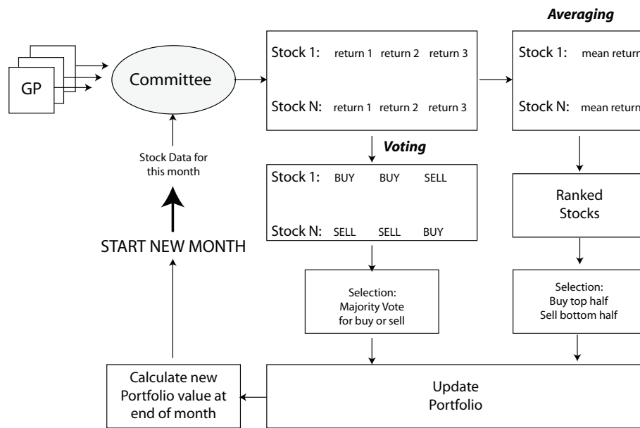
Fig. 2 The Committee in action: either Averaging or Voting.
