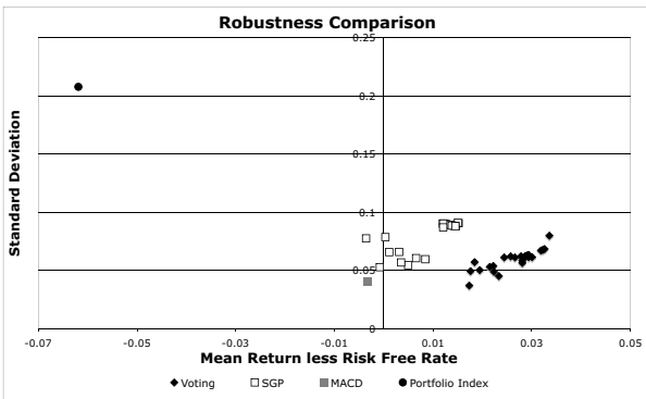
Fig. 9 Robustness comparison.
