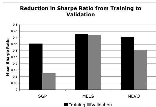
Fig. 7 Robustness measure: drop in Sharpe Ratio.
