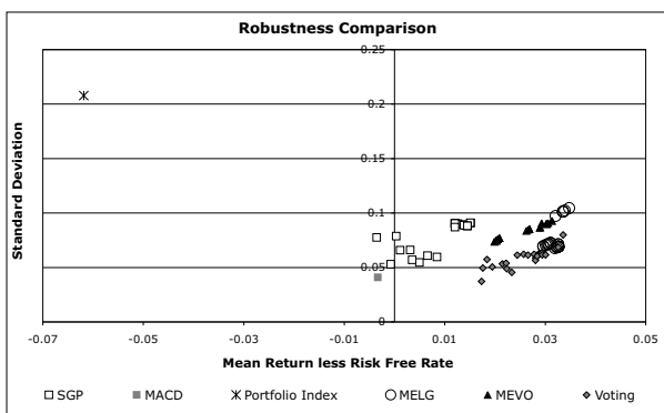
Fig. 11 Robustness comparison of all three systems.
