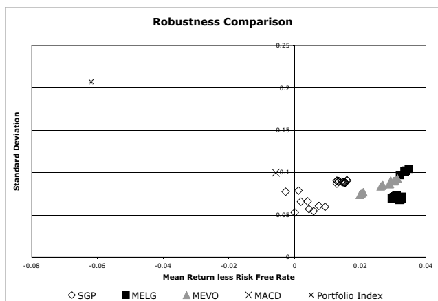
Fig. 6 Robustness comparison.
