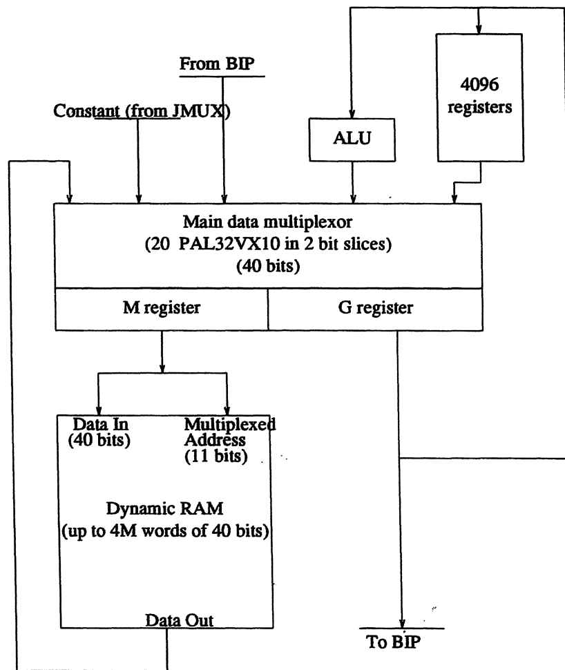
Figure 6. IMU data path
