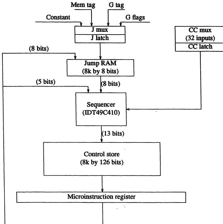
Figure 7. IMU Control Section block diagram
