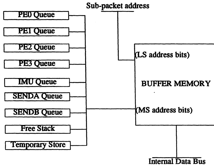
Figure 4. BIP block diagram
