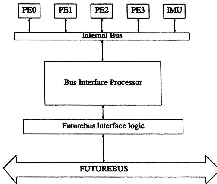
Figure 2. A GRIP board
